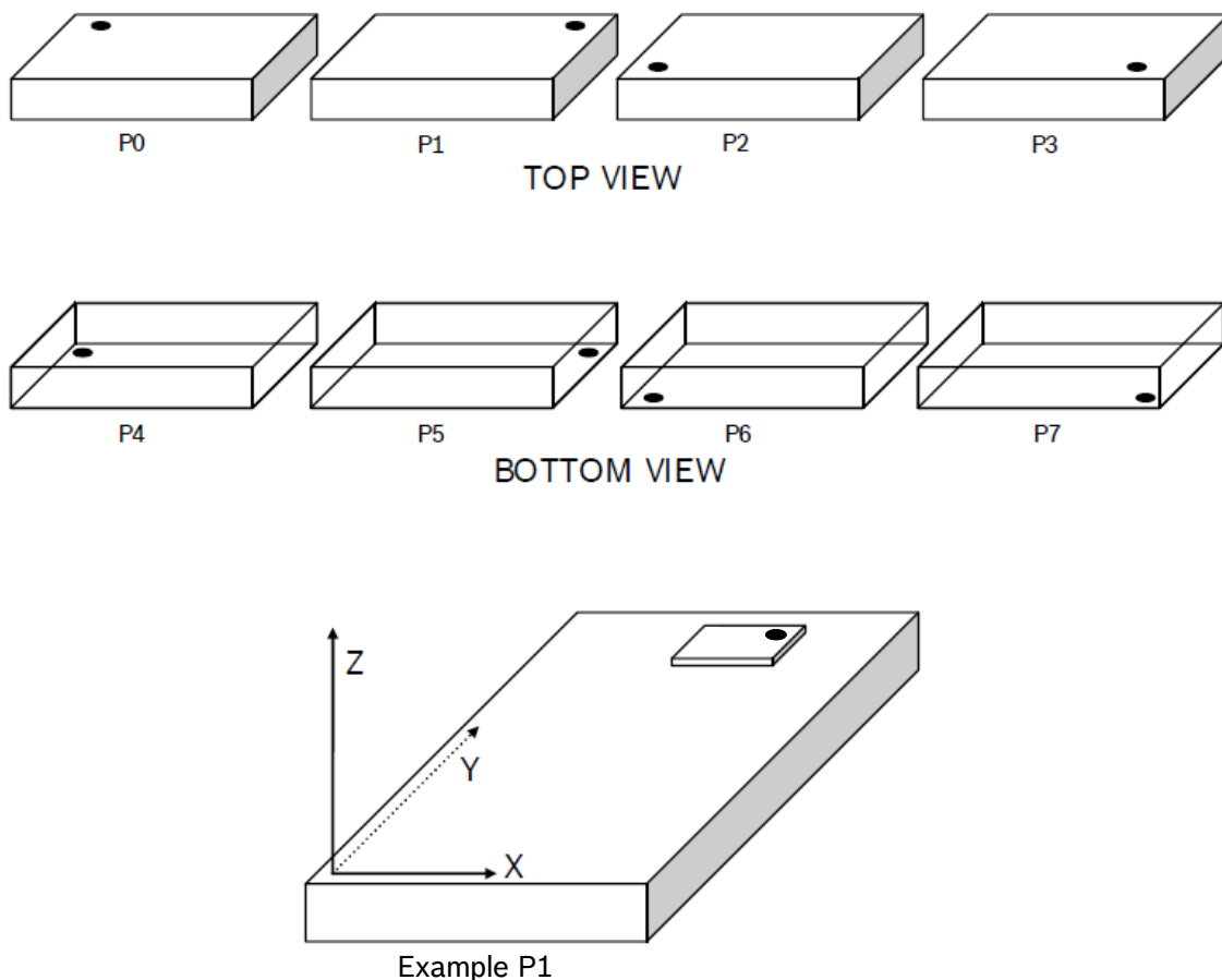
Figure 10: Placement options with respect to device orientation
